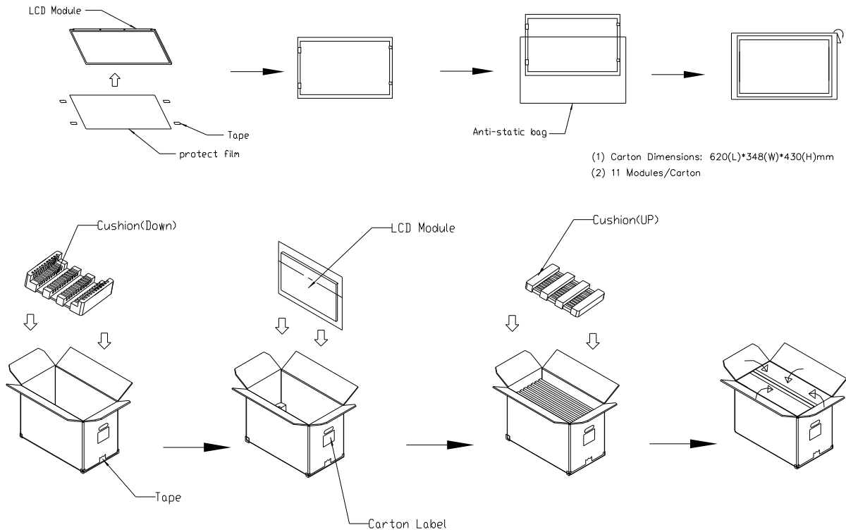
Figure 10-1 packing method
